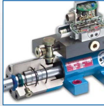
Servo Controlled Cylinder
