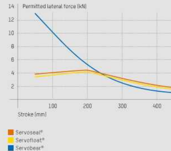
Permitted lateral forces in relation to the stroke length
