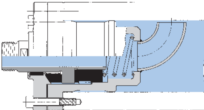
HW 125 K-24: integrated in roller trunnion at return for cooling water.
