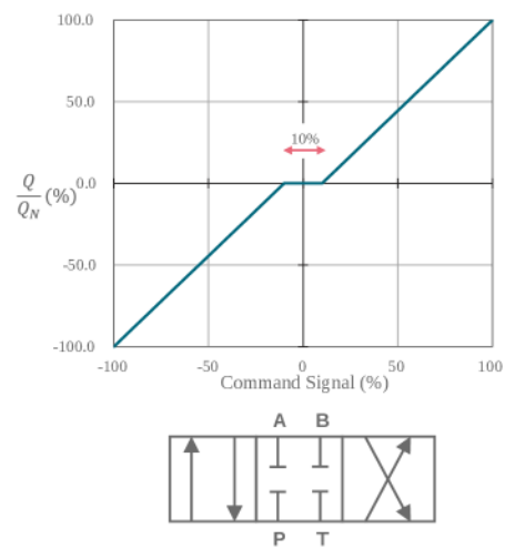
D - Deadband
