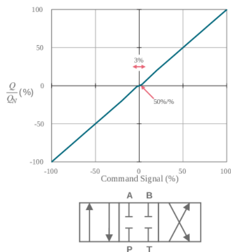
O - Overlap
