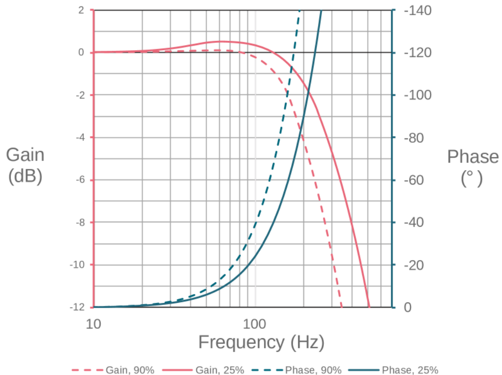
Frequency Response (1)
