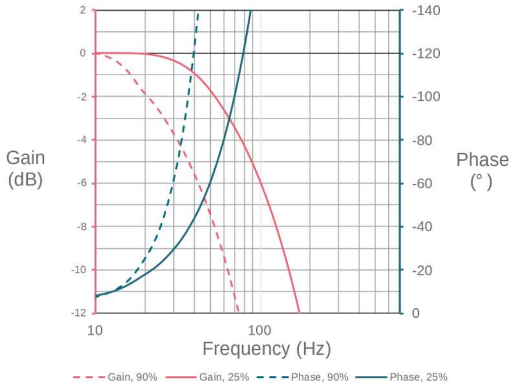
Frequency Response (1)
