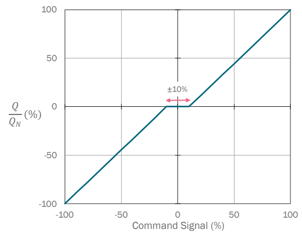
D - Deadband
